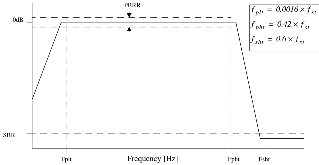
Fig 11. Telecom output frequency response
